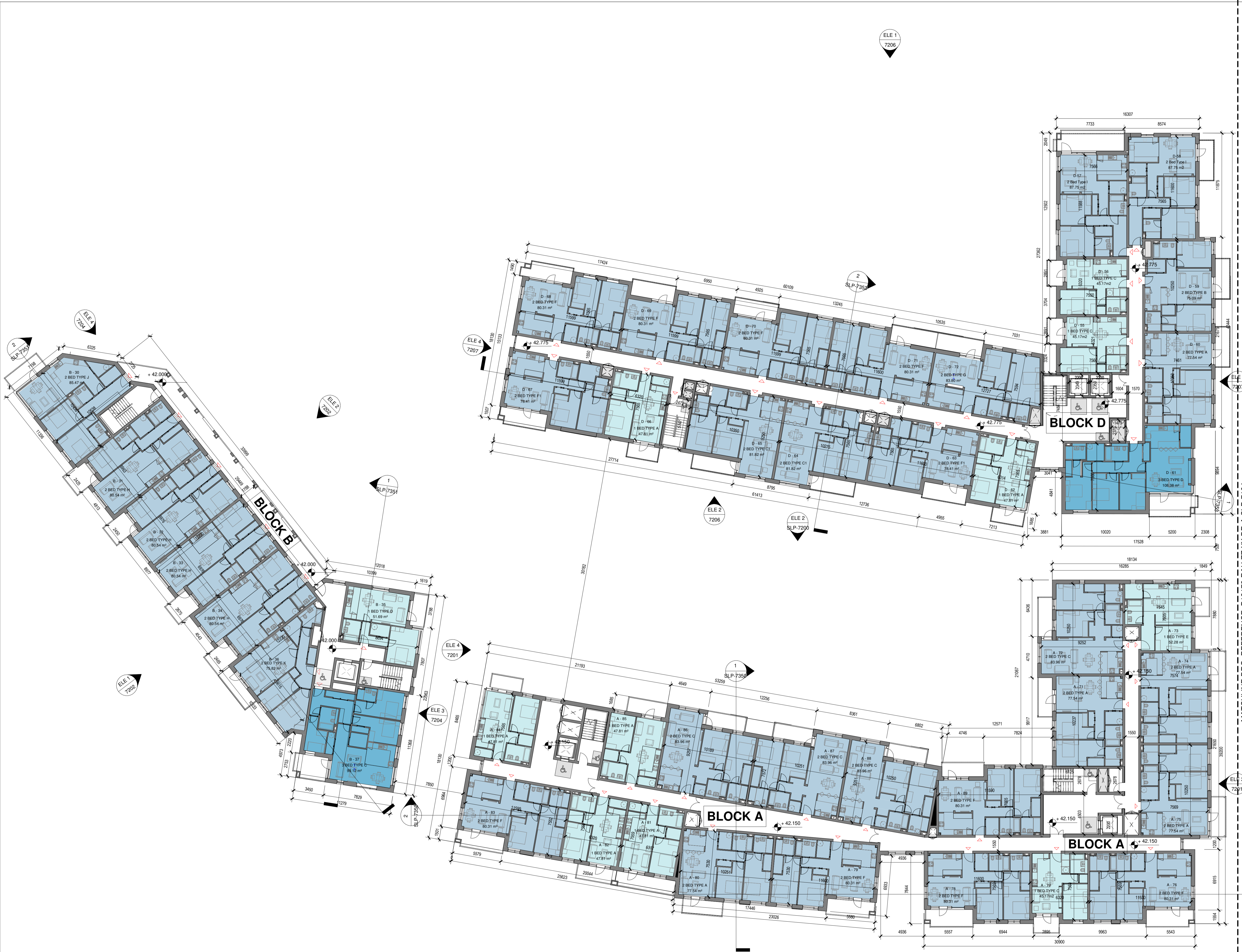
1 Floor Plan Level 04 Block A_B_C_D 1 : 200
